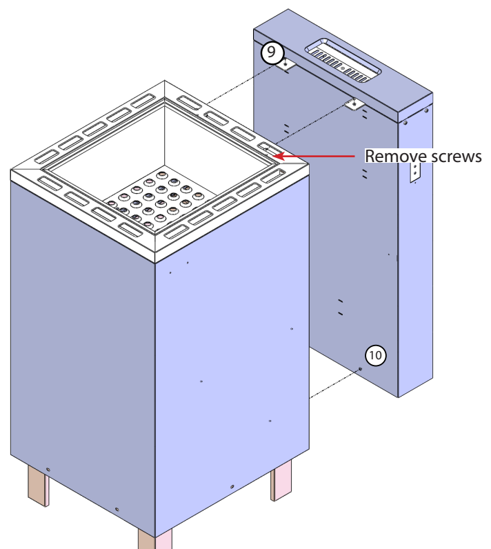
Fig 3b Sauna Heater Part diagram
